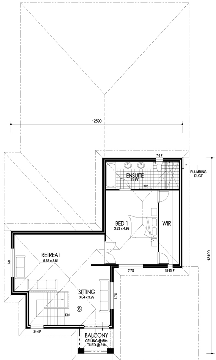
First Floor
